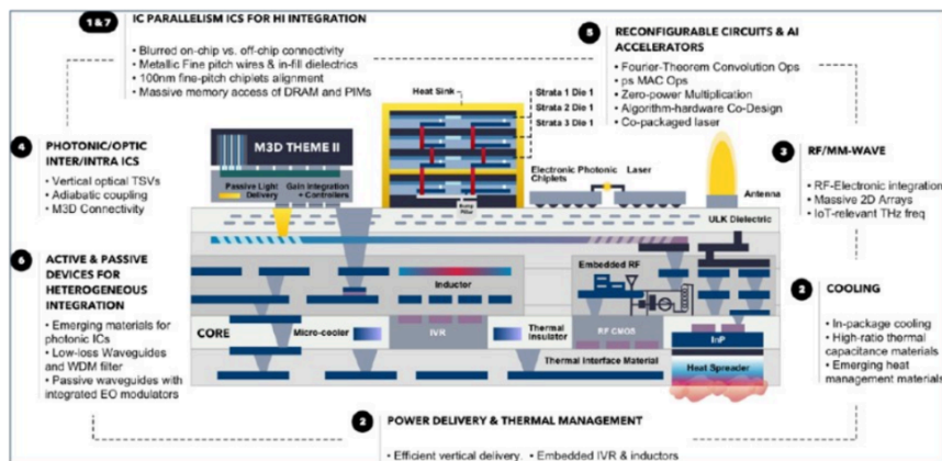
Exhibit 1: Concept of Ultra-dense Advanced Packaging
